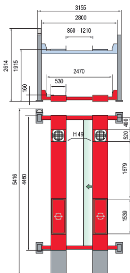
PROLIFT 440MA
